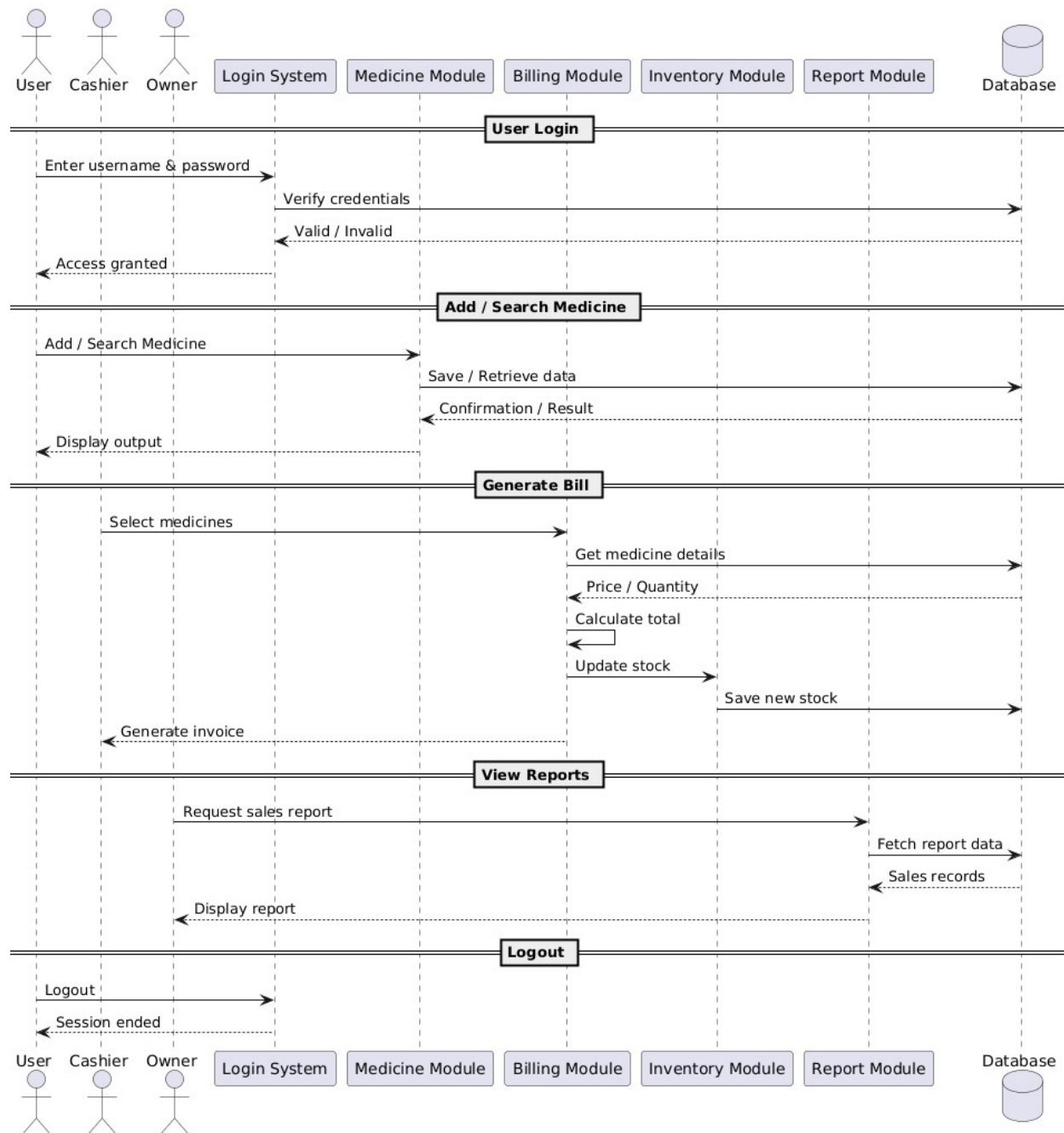
Figure 03: Sequence Diagram
